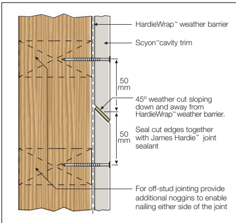
FIGURE 10 SCYON™ CAVITY TRIM BUTT DETAIL
