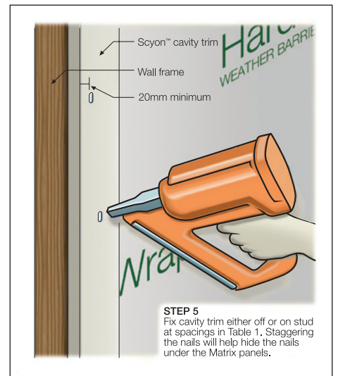
FIGURE 8 FIXING SCYON CAVITY TRIM
