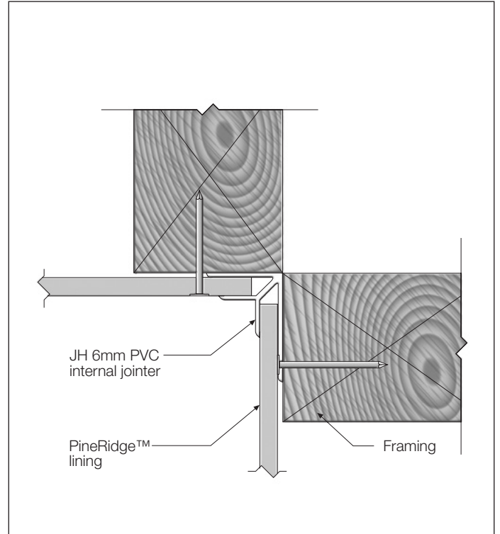
FIGURE 12 INTERNAL CORNERS
