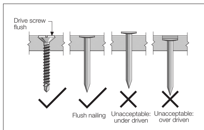
FIGURE 2 FASTENER DEPTH
