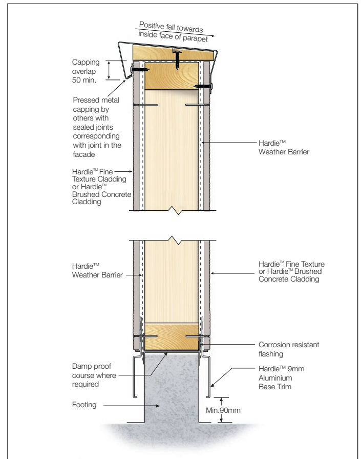
FIGURE 7 BLADE WALL
