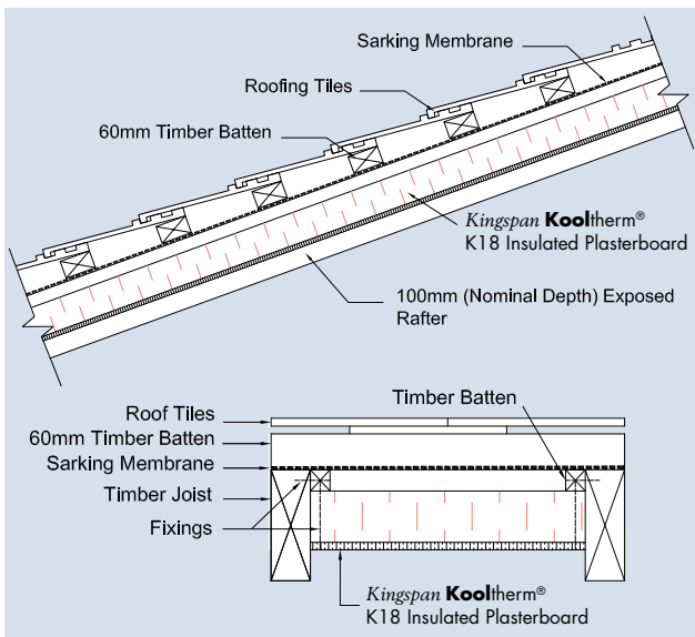
Figure 10 Side and front elevation - Raked ceiling (exposed beam) with Kingspan Kooltherm® K18 Insulated Plasterboard
